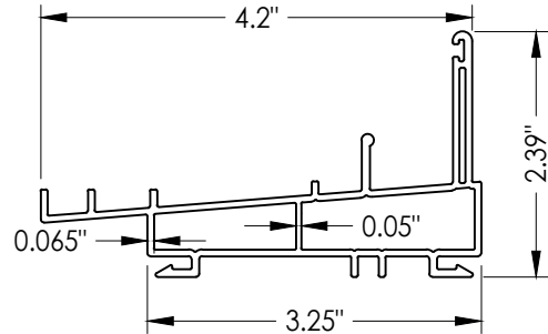
16 SLOPED SILL "DH30"
