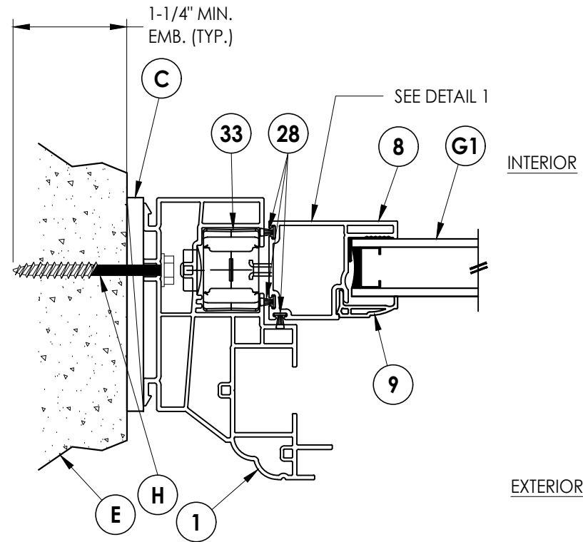
2 HORIZONTAL CROSS SECTION 2 Shown Direct to Masonry
