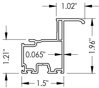
10 LIFT RAIL
