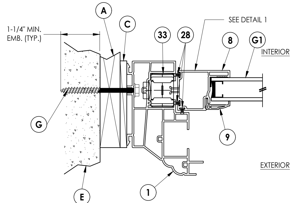
3 HORIZONTAL CROSS SECTION 2 Shown w/ 1X Buck
