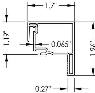
7 LOCK RAIL
