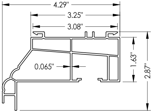
2 HEAD
