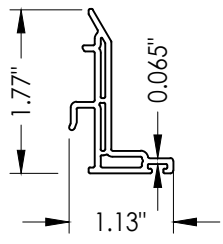
14 HEAD POCKET INSERT
