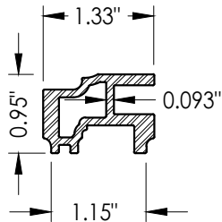
13 REINFORCEMENT
