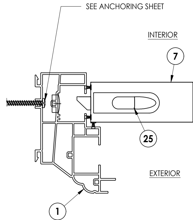
DETAIL 1
