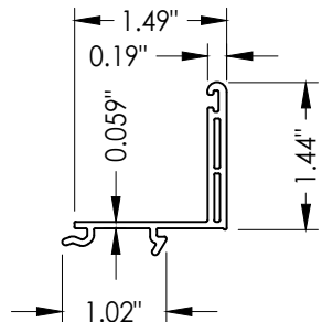
4 SILL ADAPTER
