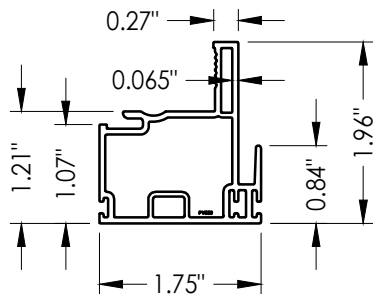
6 KEEPER RAIL
