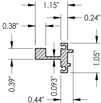
12 REINFORCEMENT
