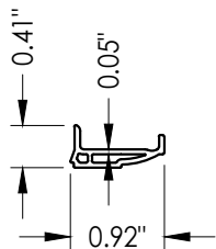
9 GLAZING BEAD
