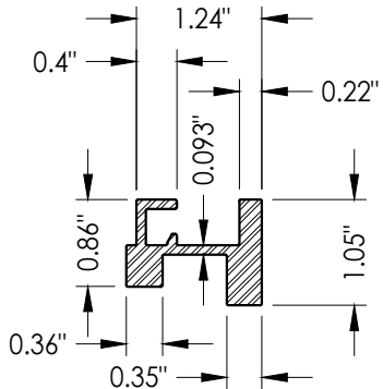
11 REINFORCEMENT
