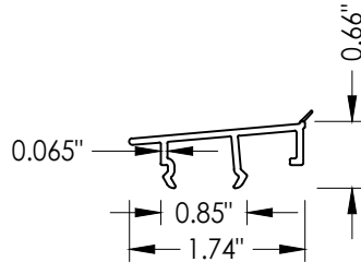
15 SLOPED INSERT
