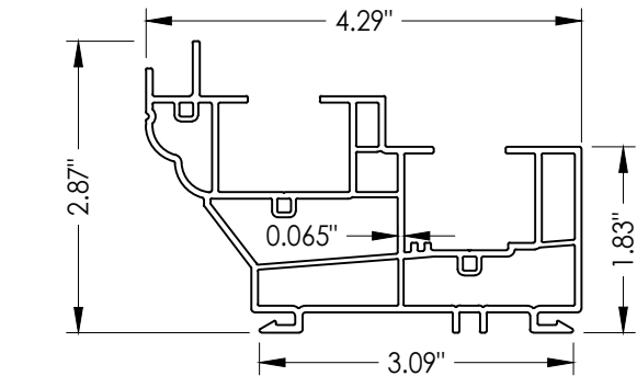
1 SLOPED SILL "DH30P"
